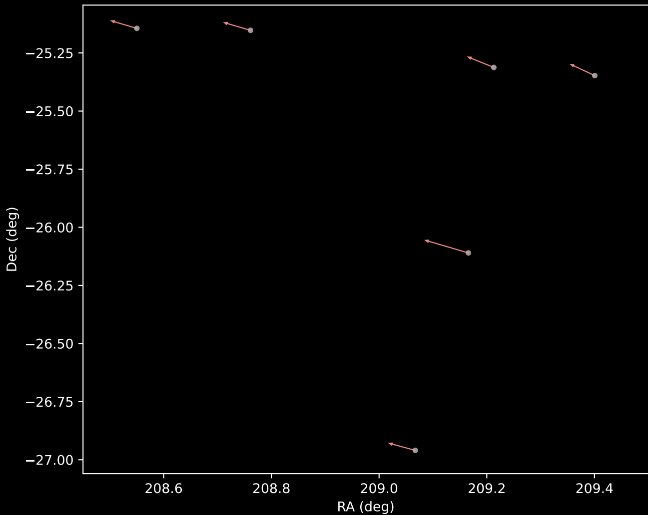
GALAH DR4 Cluster 7 Proper Motion Vectors (n=6)
