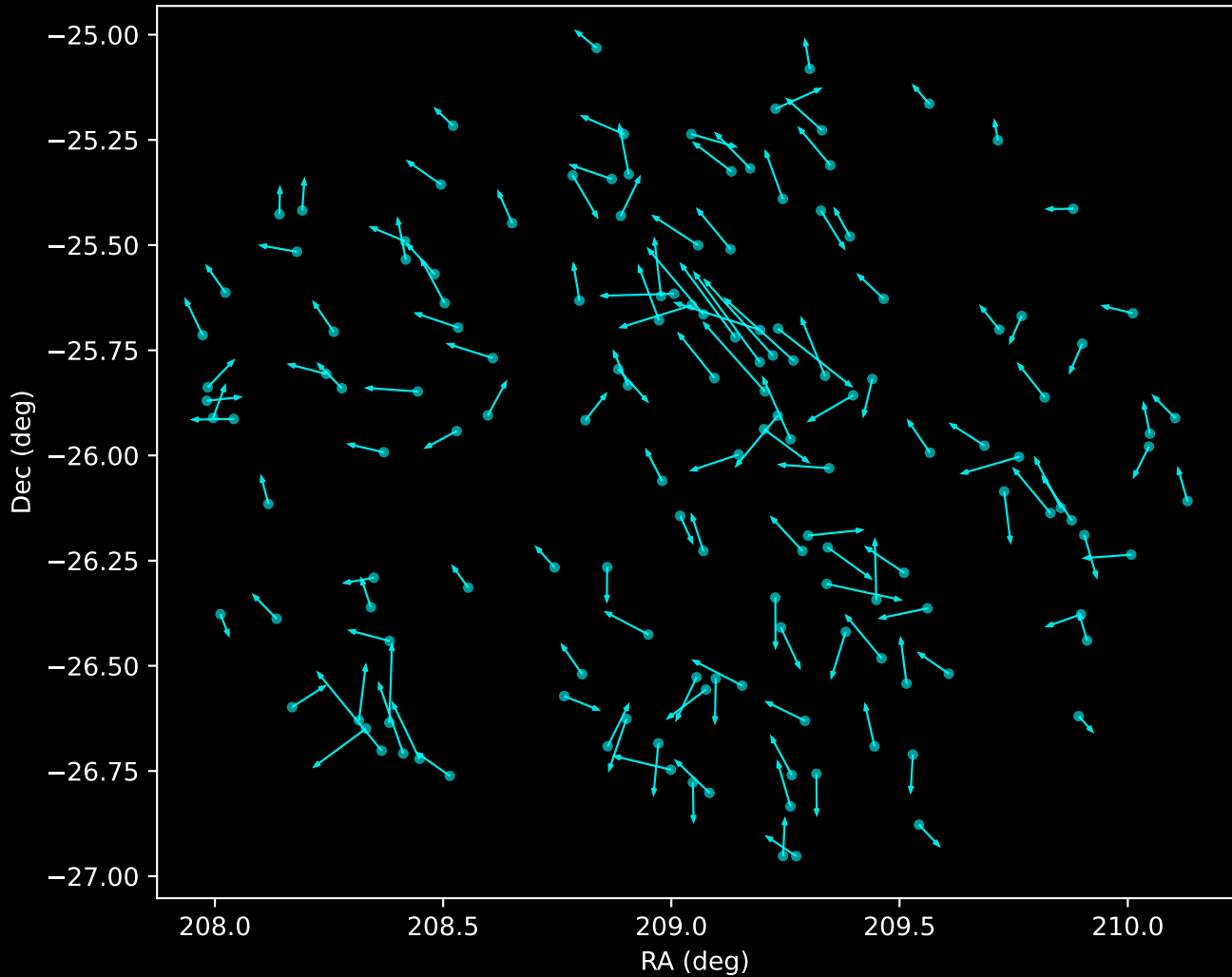
GALAH DR4 Noise Stream Proper Motion Vectors (n=148)
