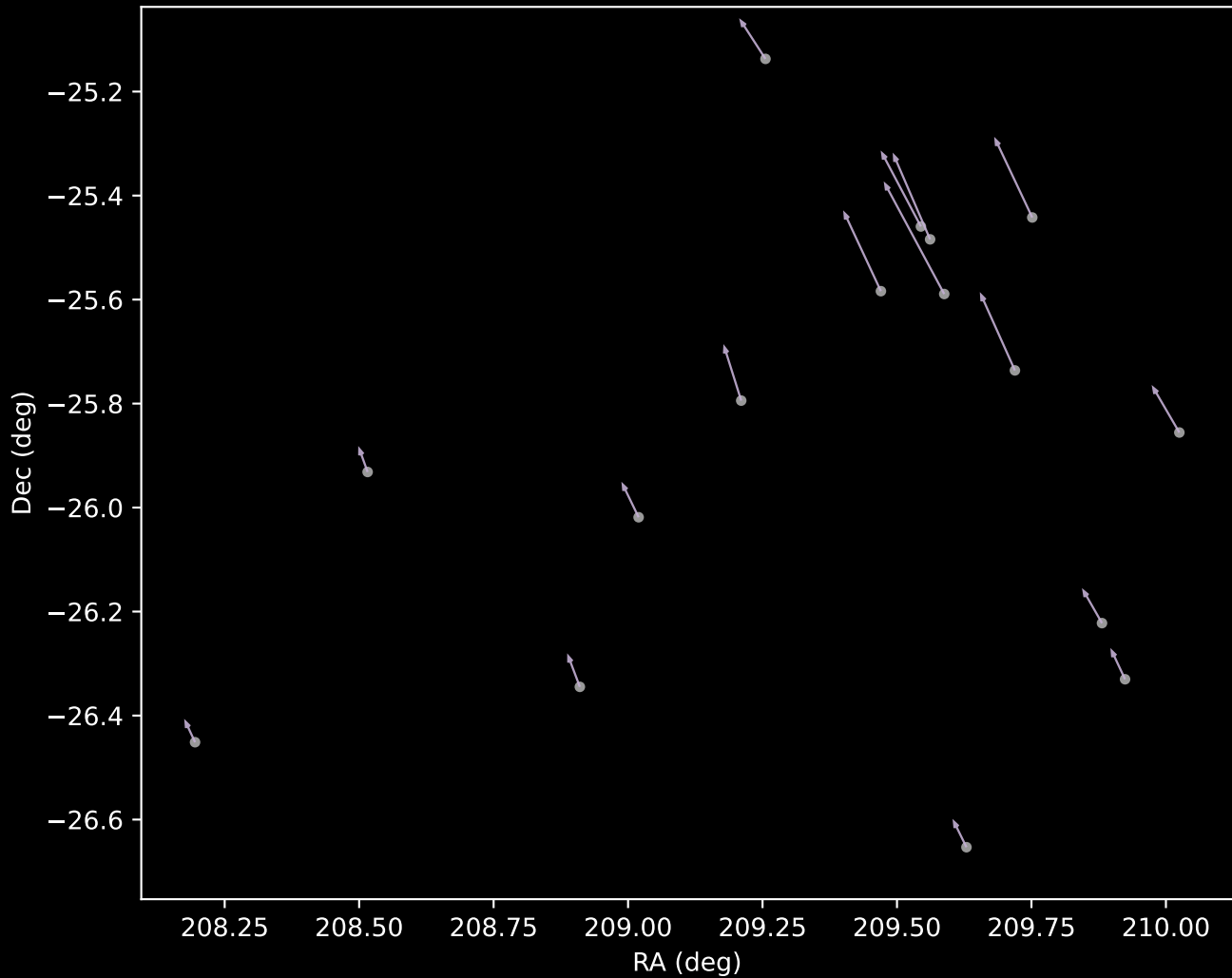
GALAH DR4 Cluster 9 Proper Motion Vectors (n=16)
