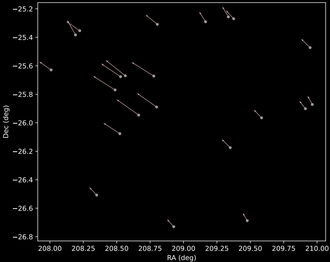
GALAH DR4 Cluster 11 Proper Motion Vectors (n=22)
