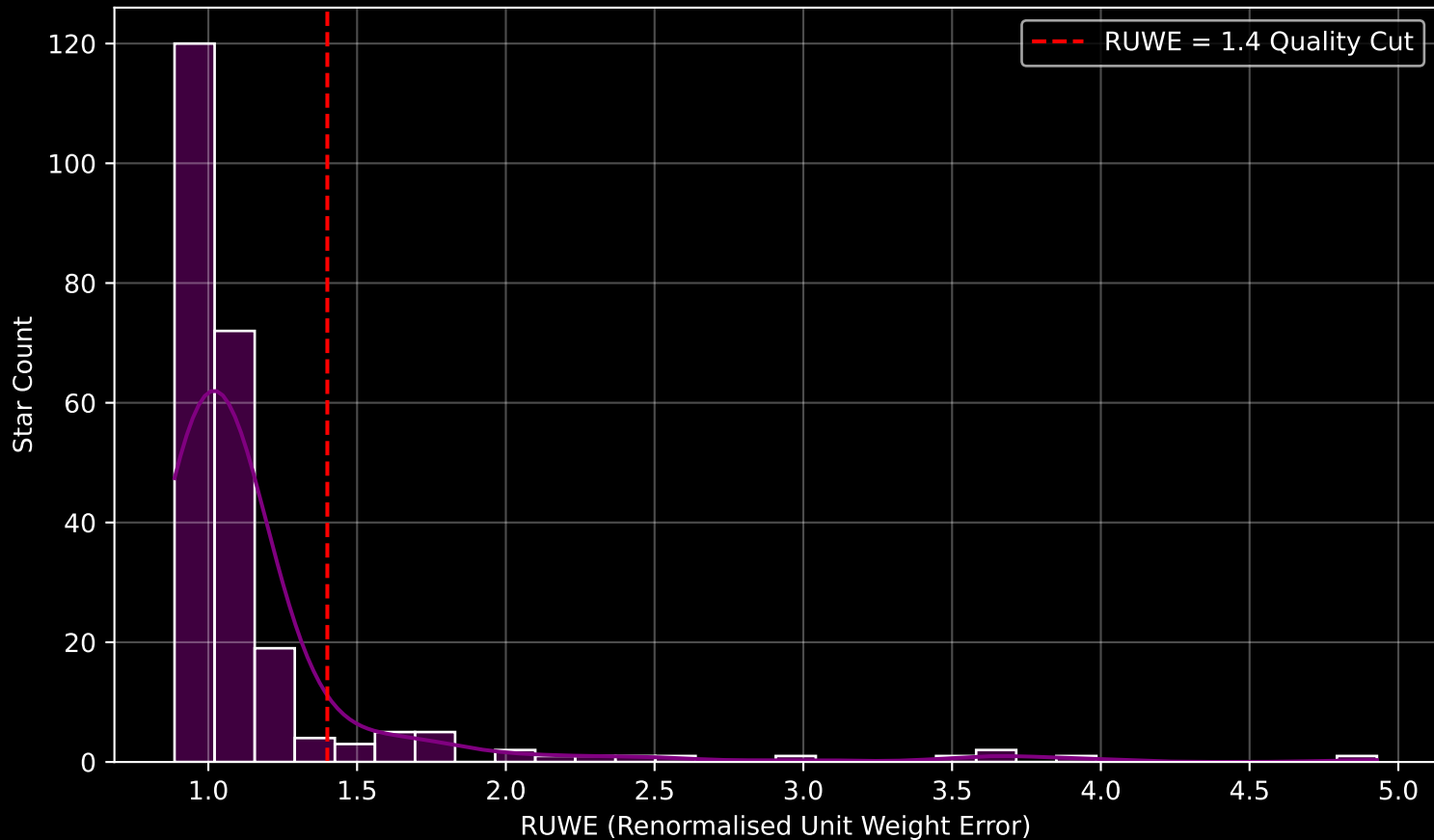
GALAH DR4 Field [8389] RUWE Distribution (n= 240)
